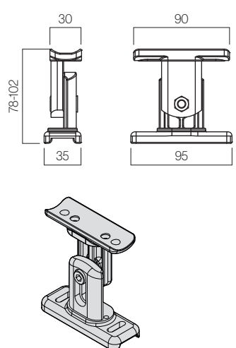
Soporte guía regulable
