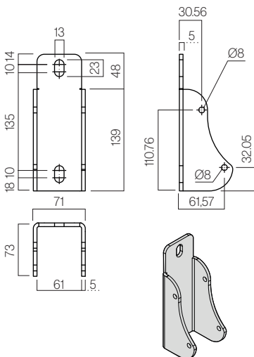
Wall support
