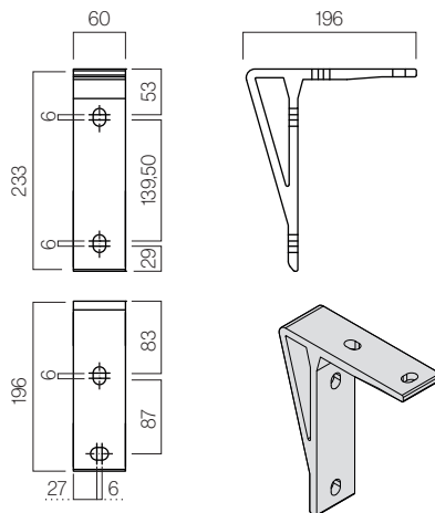
Ceiling support
