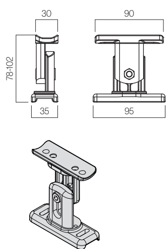
Adjustable guide support
